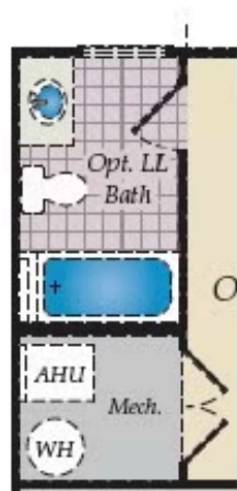
OPT. LOWER LEVEL BATH
