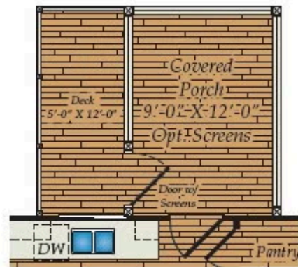
OPT. COVERED PORCH W/ DECK
