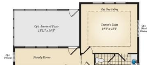
Opt. 2' Rear Extension with Opt. Screened Patio
