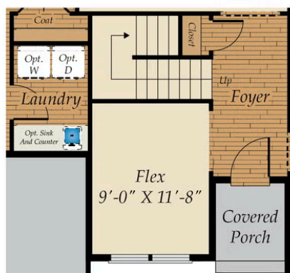
FIRST FLOOR W/OPT. 2ND FLOOR & 2-CAR GARAGE
